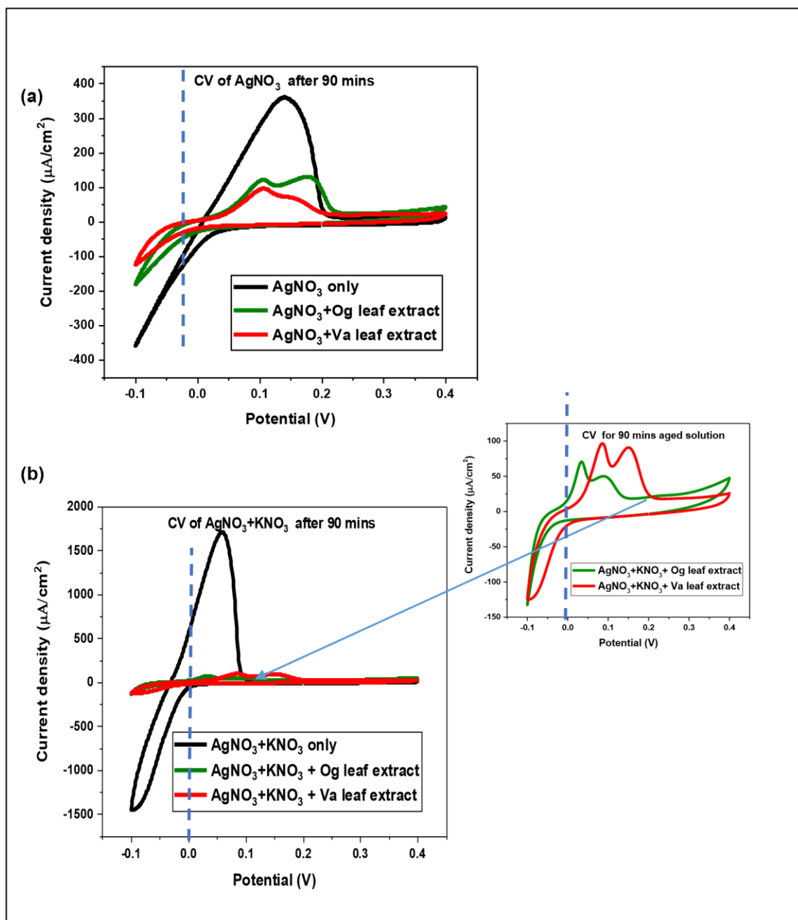
Figure 4: CV plots with and without leaf extracts after ageing for 90 minutes. CVs done in (a) 5 mM \text{AgNO}_3 and (b) 5 mM \text{AgNO}_3 + 0.1 \text{ M KNO}_3 solution at 10 mV/s. Figure (4b) inset shows enlarged CVs in the leaf solutions for clarity.
