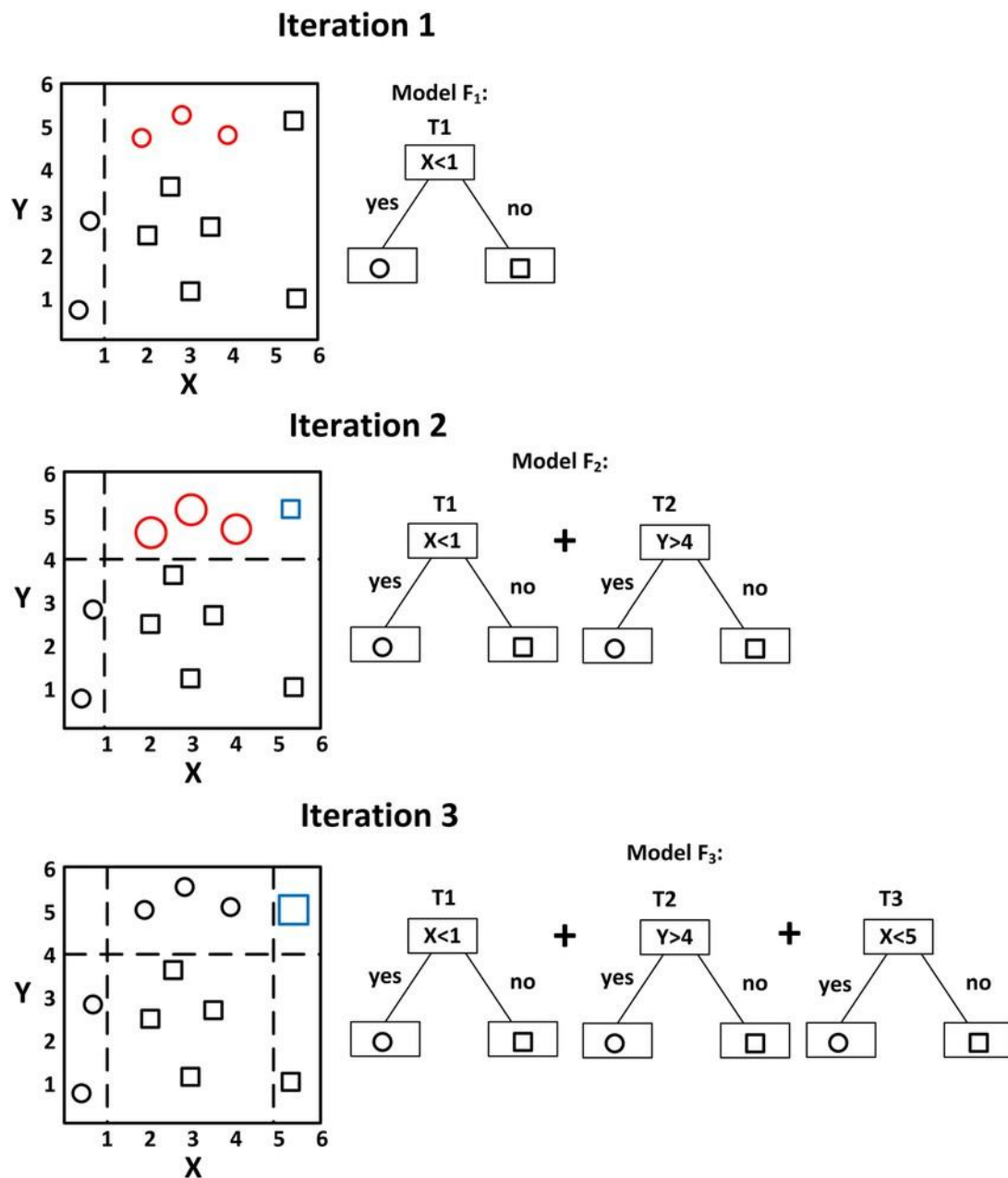
Figure 5. Boosting Method
