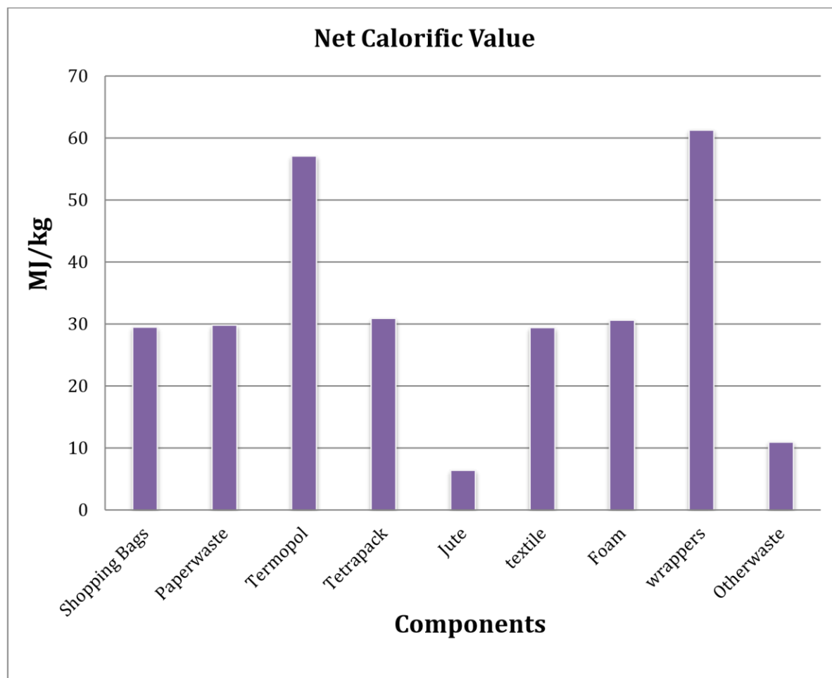
Figure 2: Net calorific value 3.6 Quality Characterization of RDF
